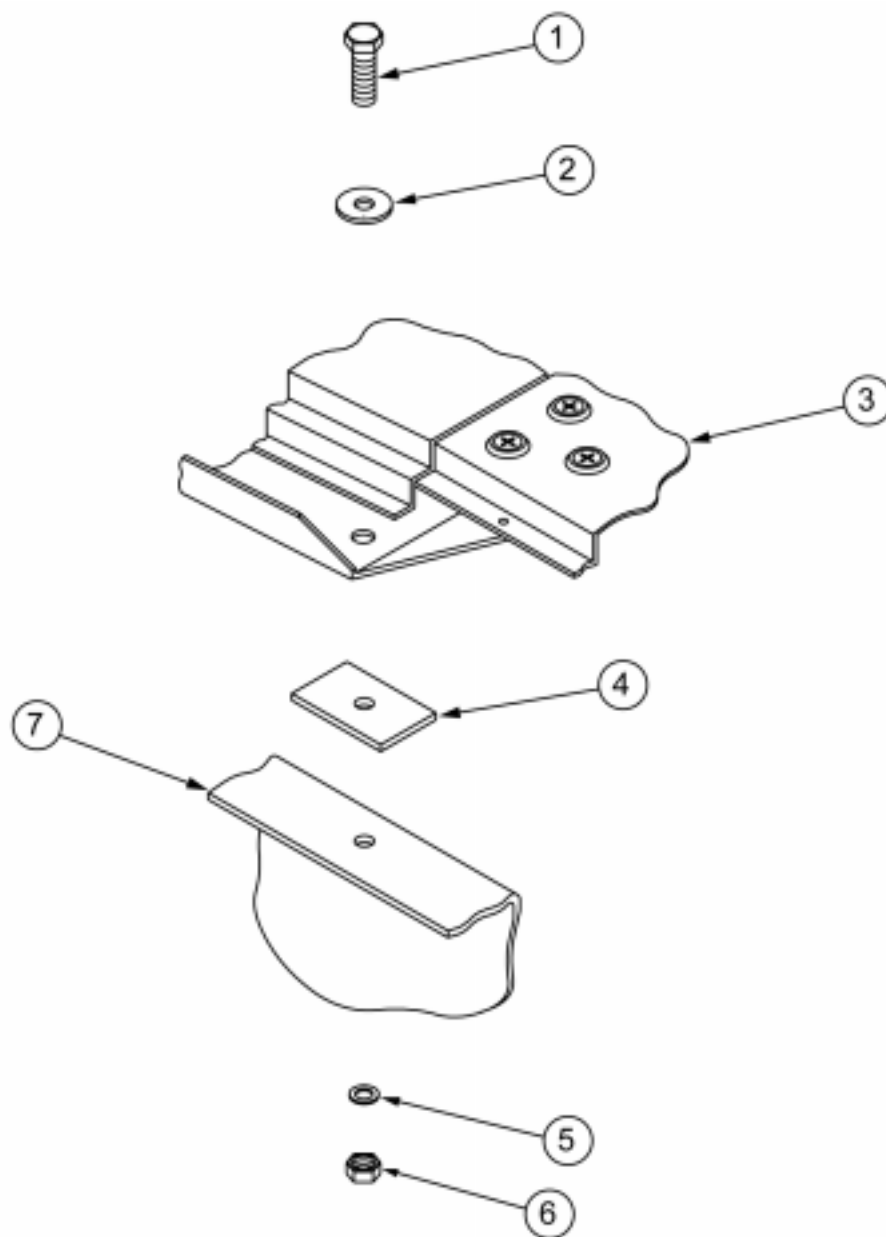
Figure 2: Cab Mount—Position 2 (Passenger Side Shown)
