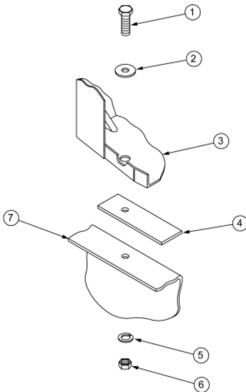
Figure 1: Cab Mount—Position 1 (Passenger Side Shown)
