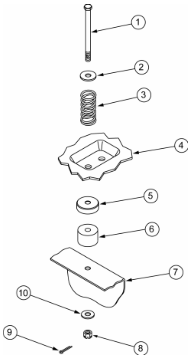
Figure 4: Cab Mount—Positon 4 (Passenger Side Shown)
